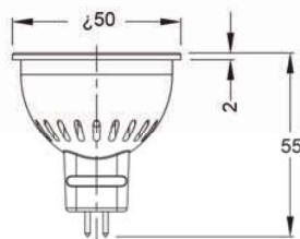
Dimensional Diagrams
