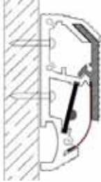
Hed Lite single wall mount system shown with optional clear shield
