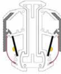
Rail Lite double rail mount system shown with optional clear shield
